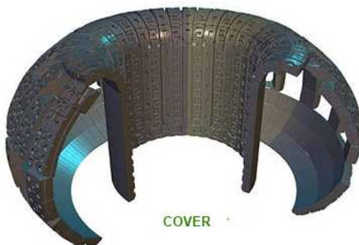
Tritogenic blanket geometry (ITER website)
